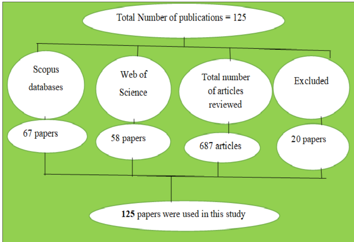
Figure 2: Flowchart for the selection of literature
