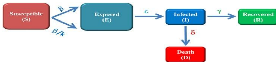
Figure 4. Schematic Presentation of the SIERD Model
