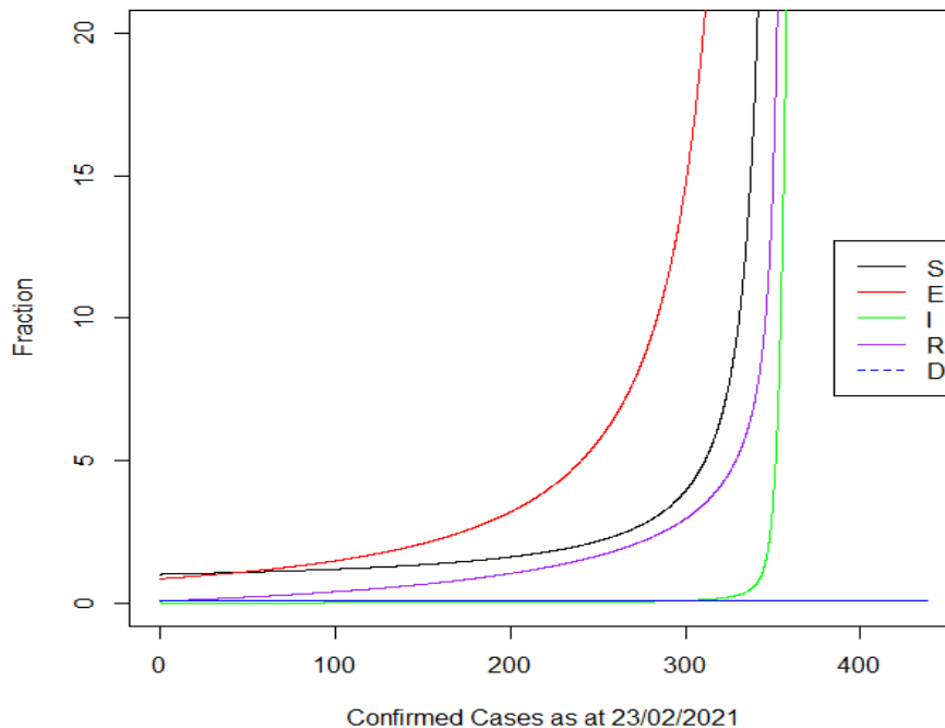
Figure 4. Graphical Representation of the SIERD Model Rate of COVID-19 in Africa (Source: Authors’ Computation (2021))
